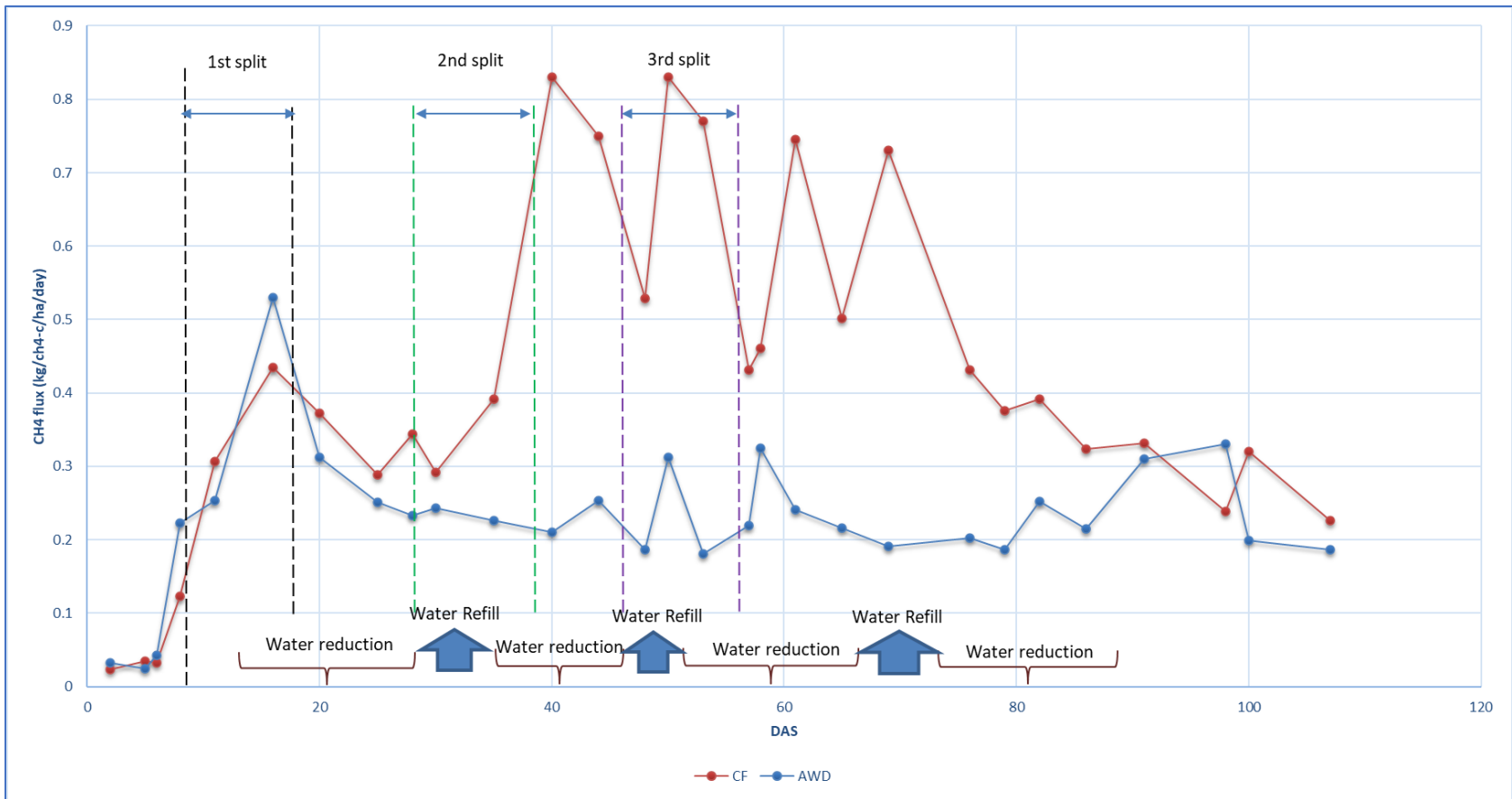
Effect of Continuous Flood (CF) and Alternate Wetting and Dry (AWD) Irrigation on Methane Emission on Rice Crop in Glasshouse Experiment
