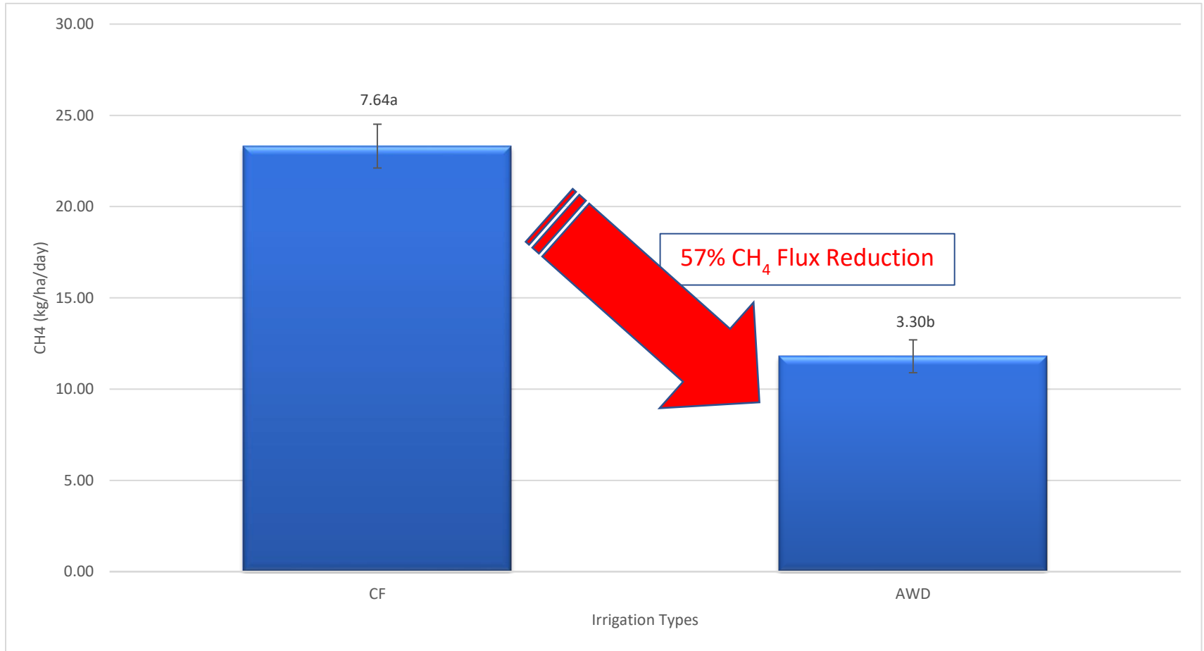
Cumulative CH 4 fluxes over growing season between CF and AWD irrigation on Rice Crop in Glasshouse Experiment
